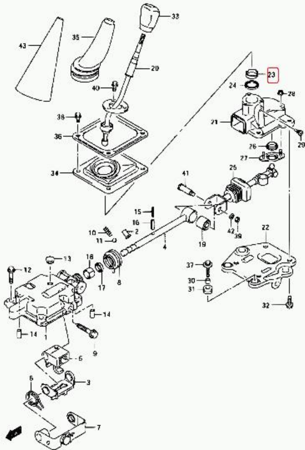
JB627W E.33_039 GEAR SHIFT CONTROL (MT)
