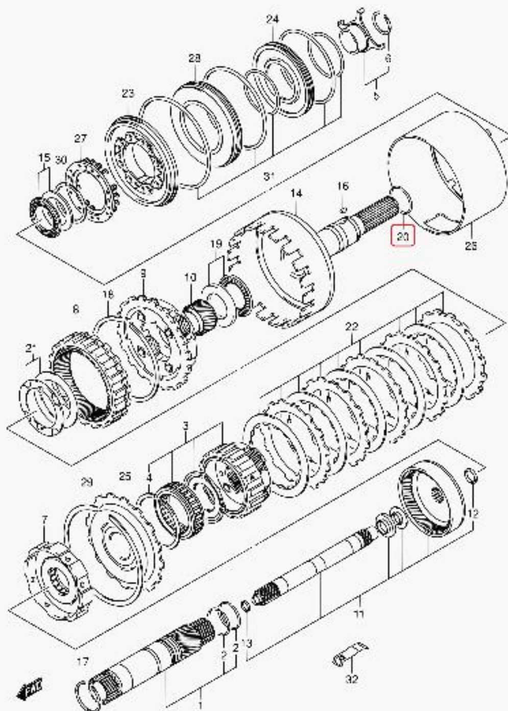
JB420W-4 E22 107 AT PLANETARY GEAR (JB420W, B424W)
