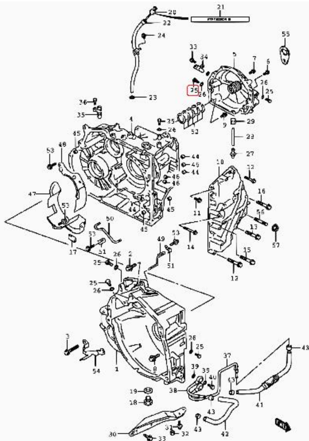
SY413-7 E01_099 4AT TRANSMISSION CASE (4AT:SY416,SY418)
