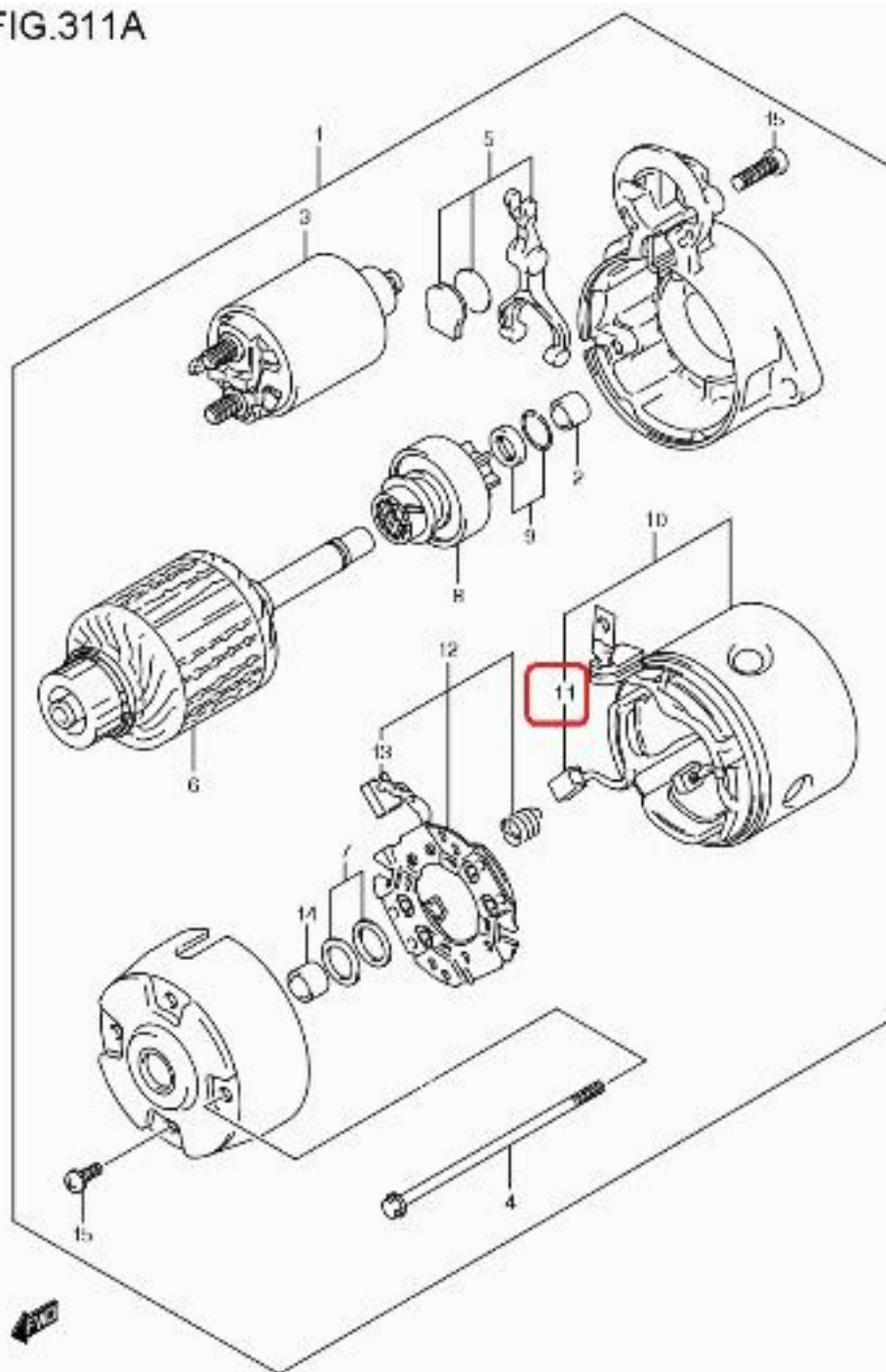
JF3W 7_311A STARTING MOTOR
