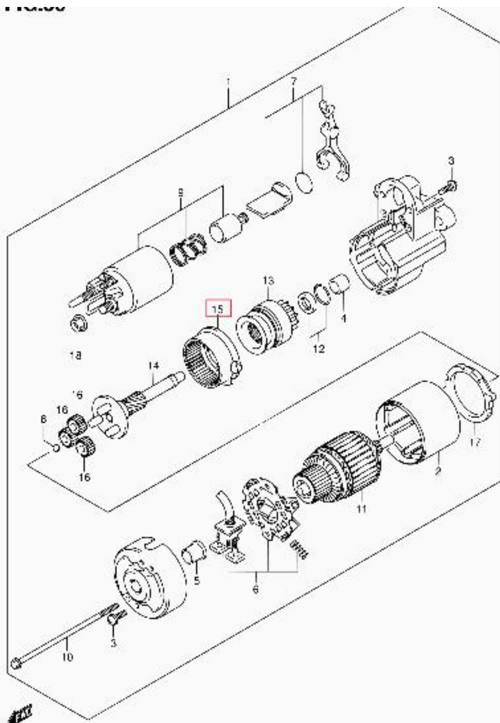
SM413V-5 E22 086 STARTING MOTOR (4)
