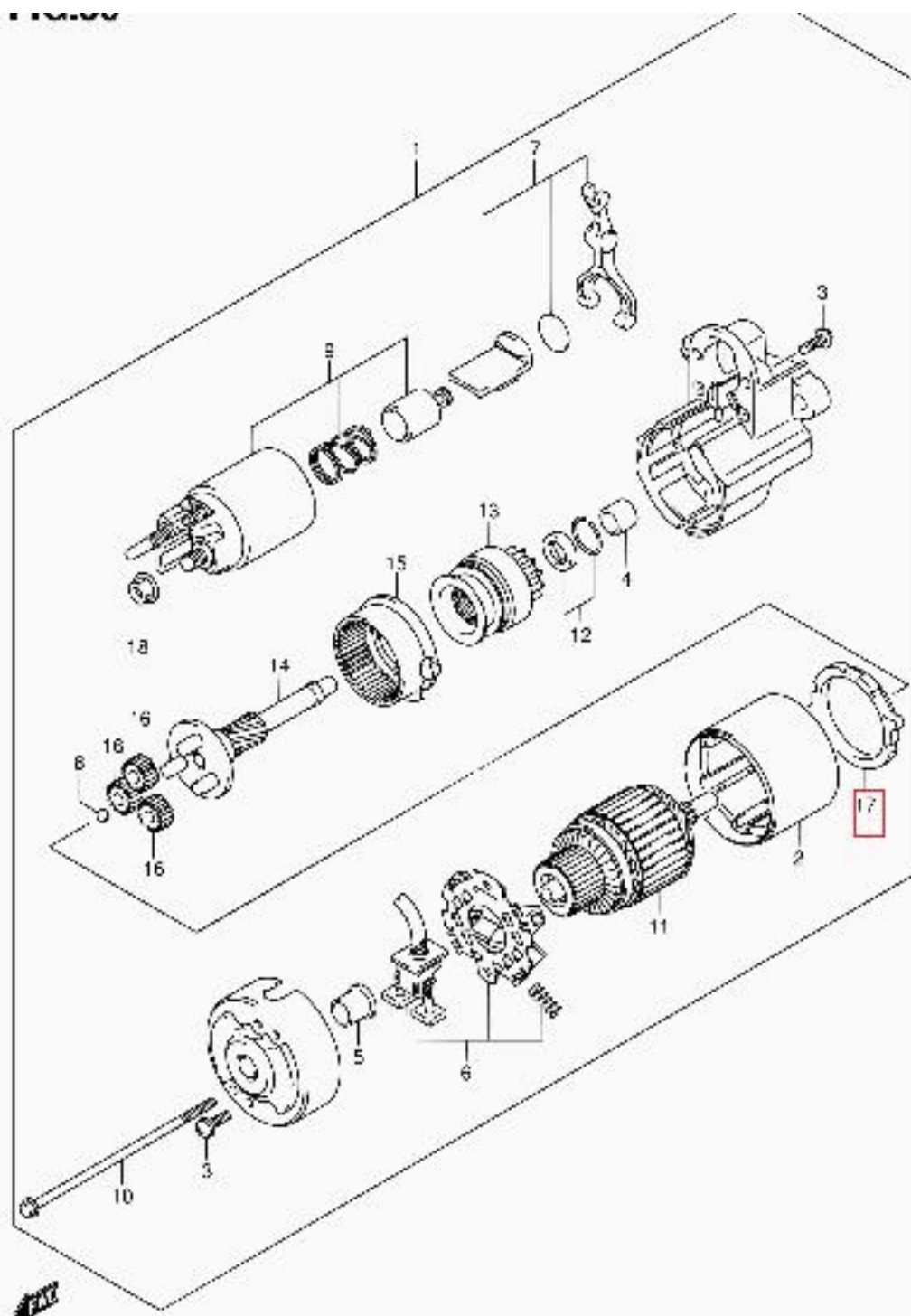
SA413V-5 E22 086 STARTING MOTOR (4)
