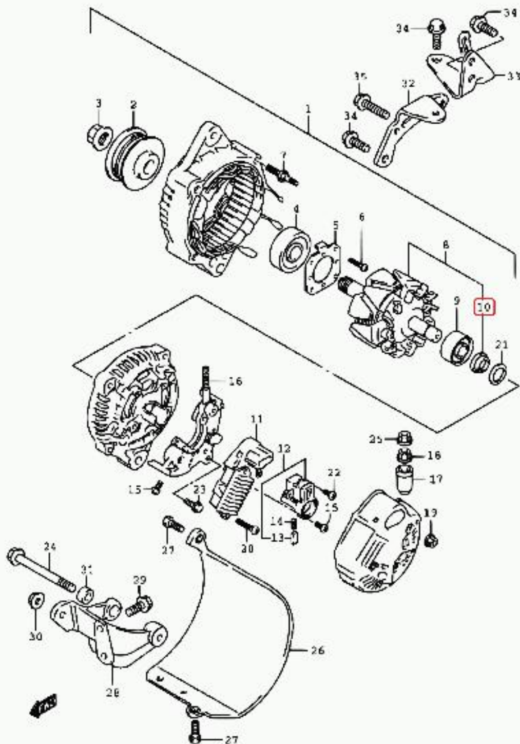
SY413-7 E01_132 GENERATOR (SY413, SY416)
