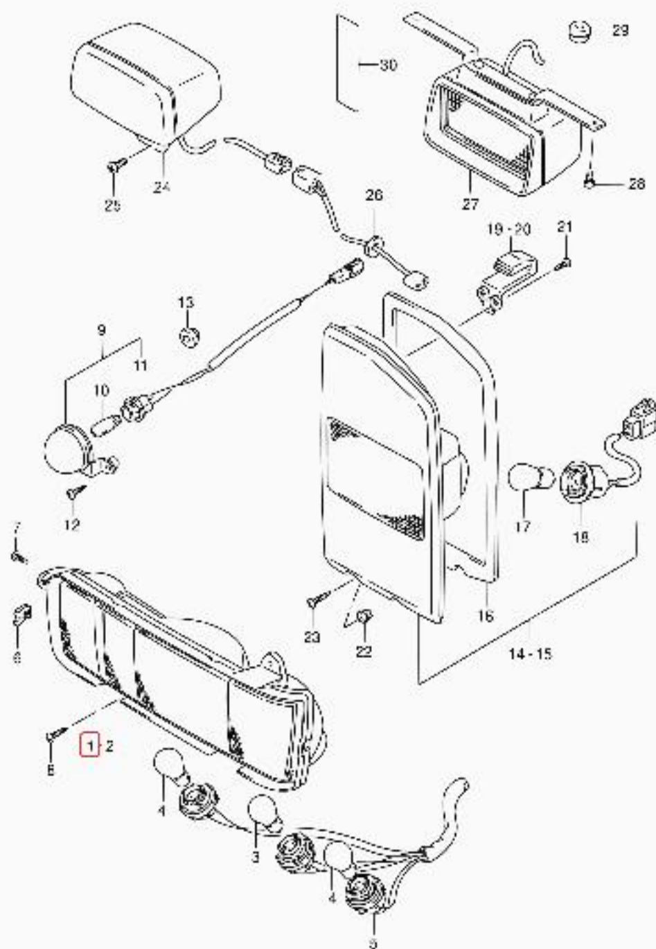
SE416 3DR E01 16' REAR LAMP (2)
