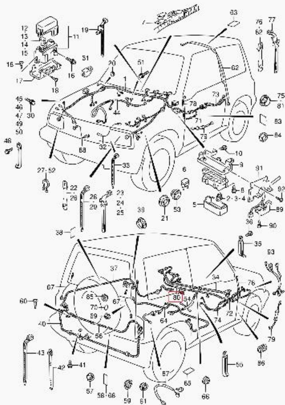
SE416 3DR E01 163 WIRING HARNESS (1)
