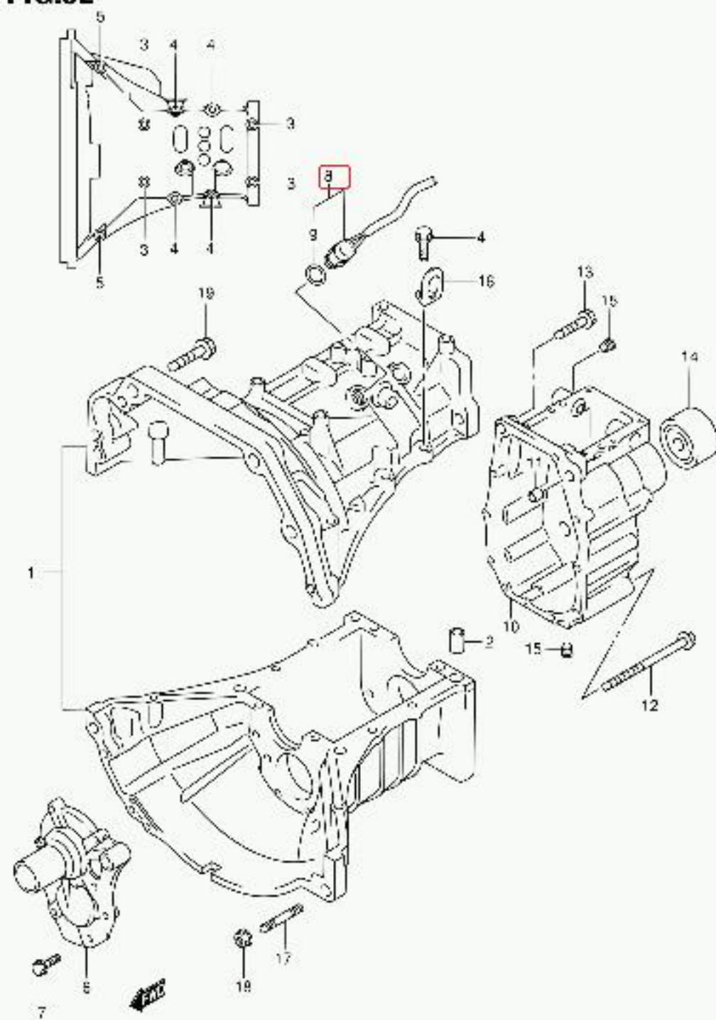
SN413V-2 E22 052 MT TRANSMISSION CASE (MT:SN413V)
