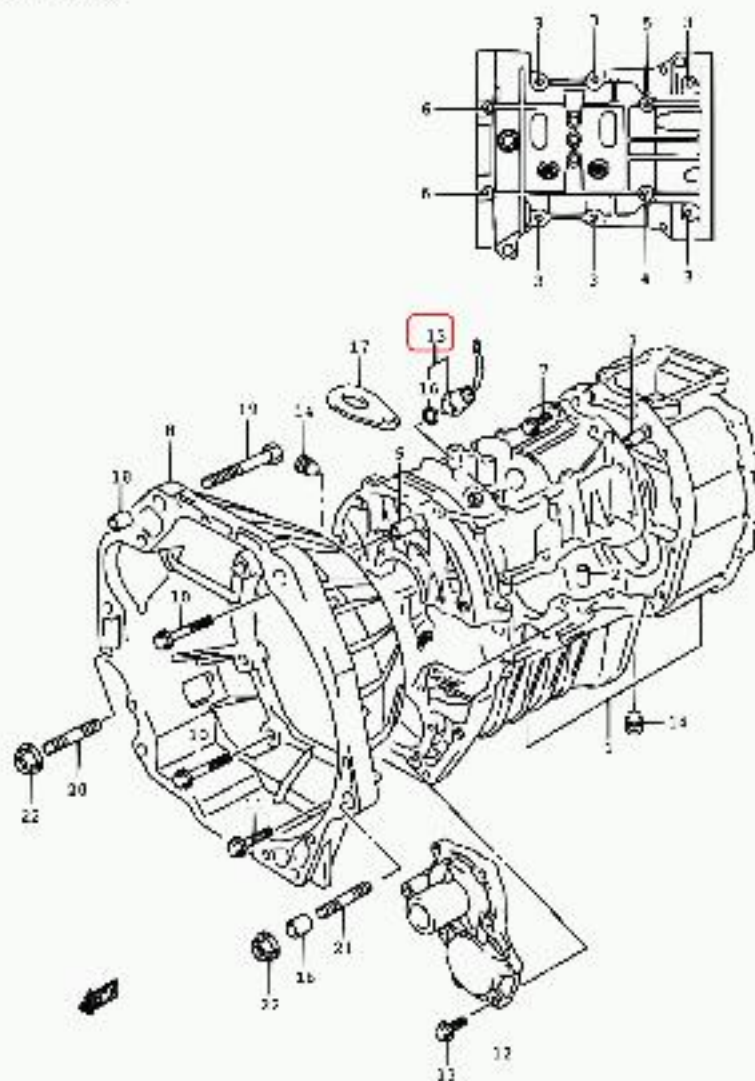
sq42cm-2 x22_108 MT TRANSMISSION CASE (MT:SQ42CM)
