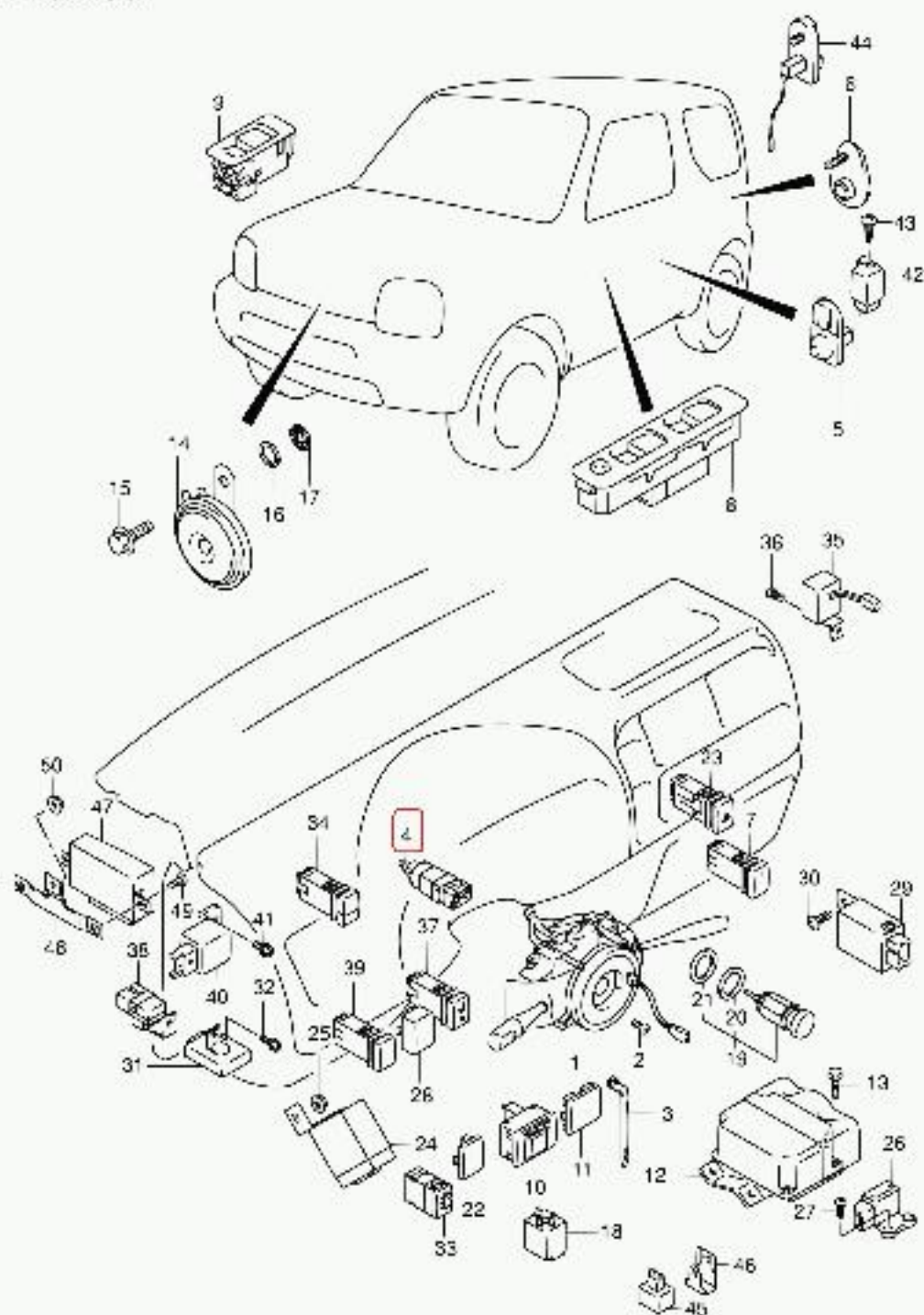
SA413V-2 E22 105 ELECTRICAL CONTROL (LHD)
