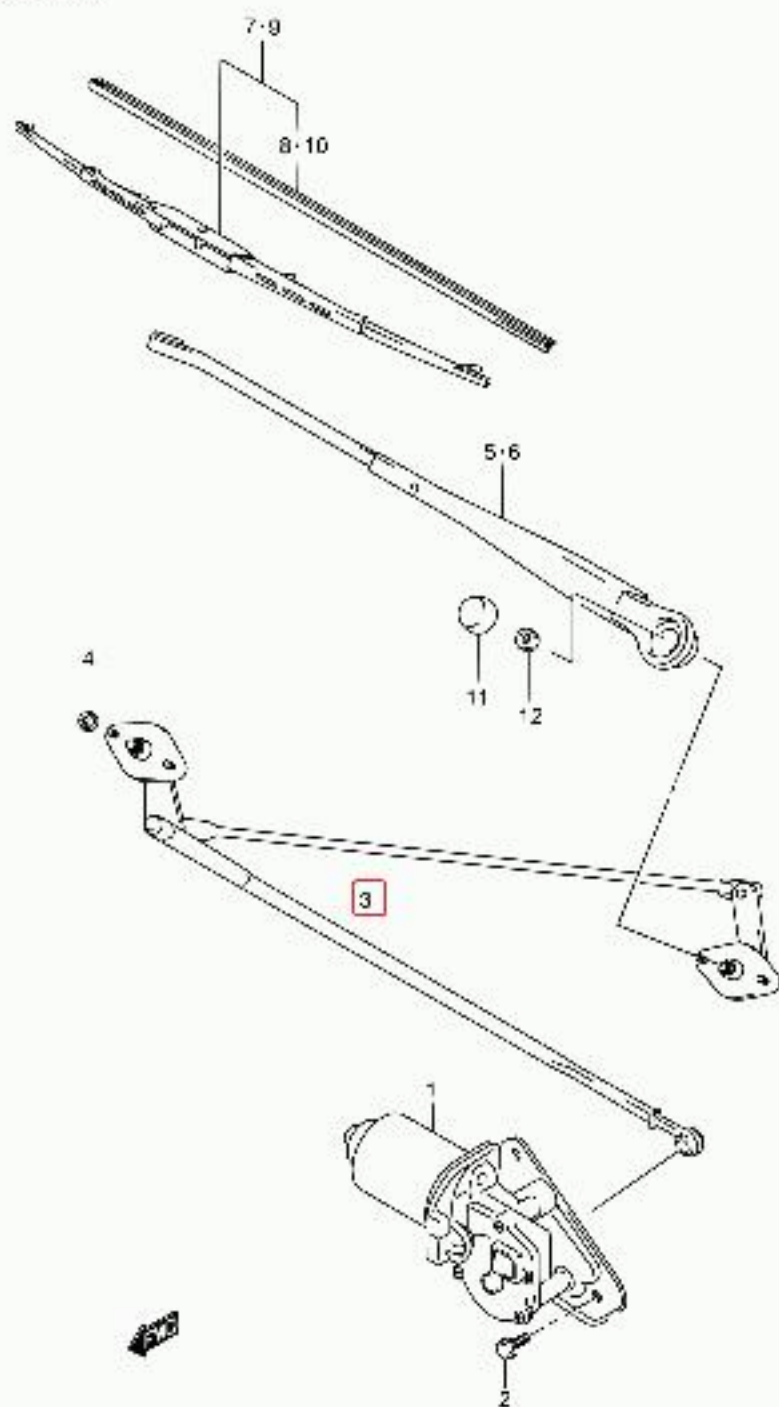
SM413V-2 E22 108 FRONT WINDOW WIPER (LHD)
