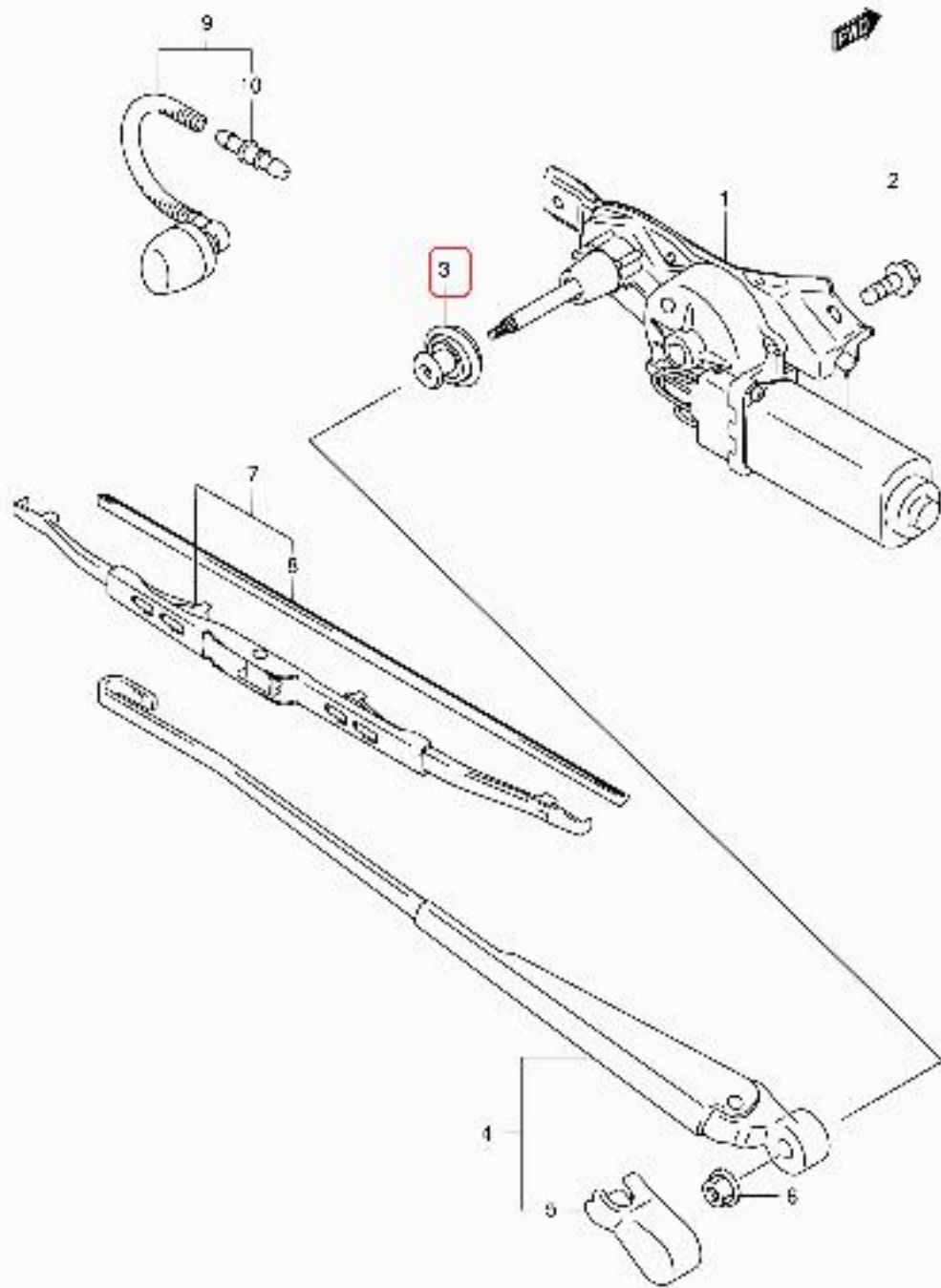
RC413 E35 057 REAR WINDOW WIPER
