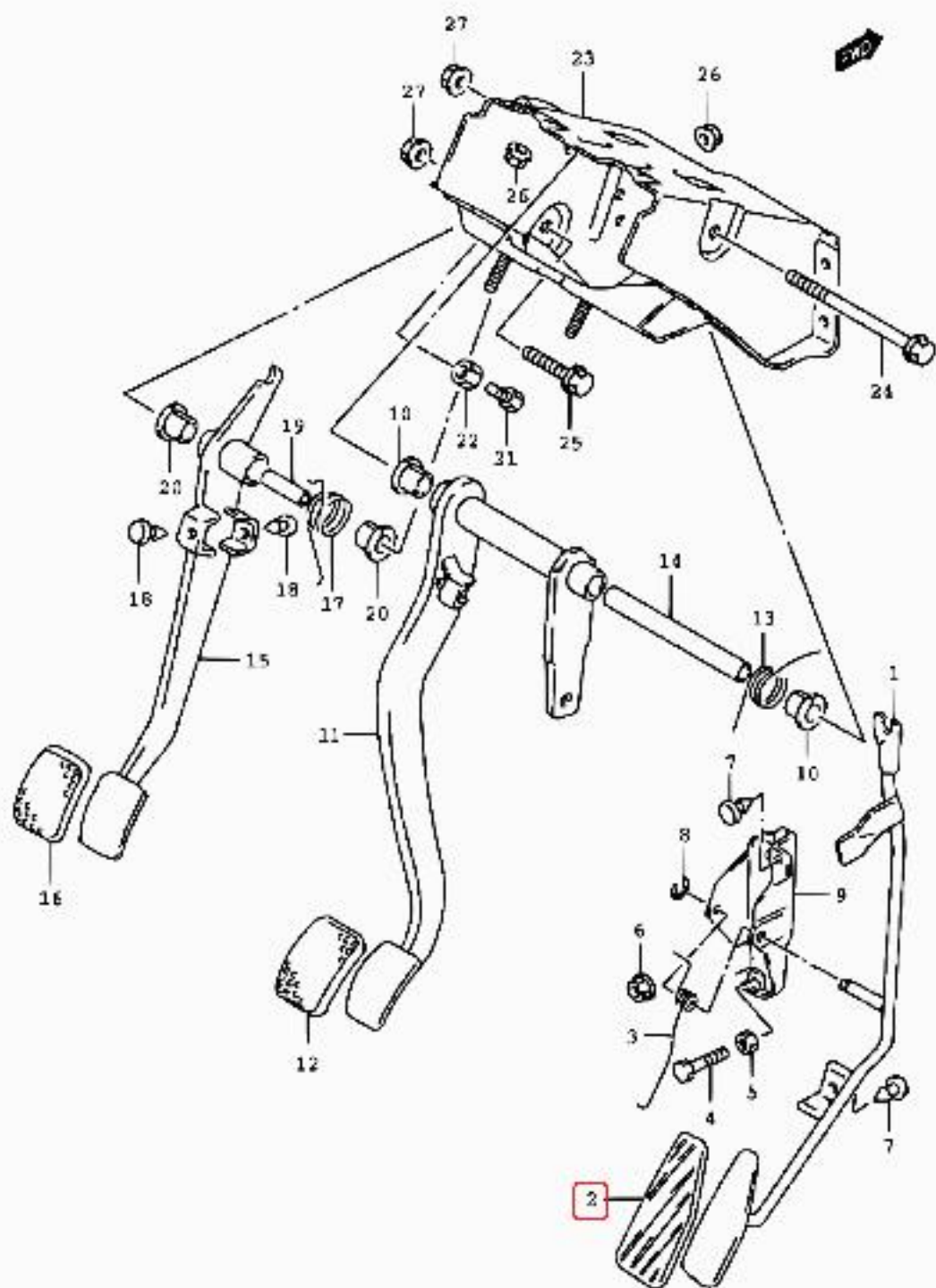
SY413-7 E01_199 PEDAL/PEDAL BRACKET (LHD:MT:2WD)
