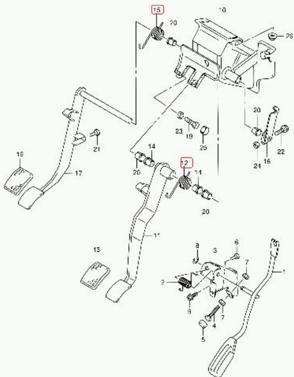
SM413V-2 E22 138 PEDAL/PEDAL BRACKET (LHD/MT)
