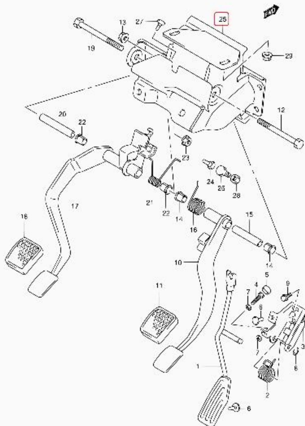
SM413V-2 E22 141 PEDAL/PEDAL BRACKET (RHD VT)
