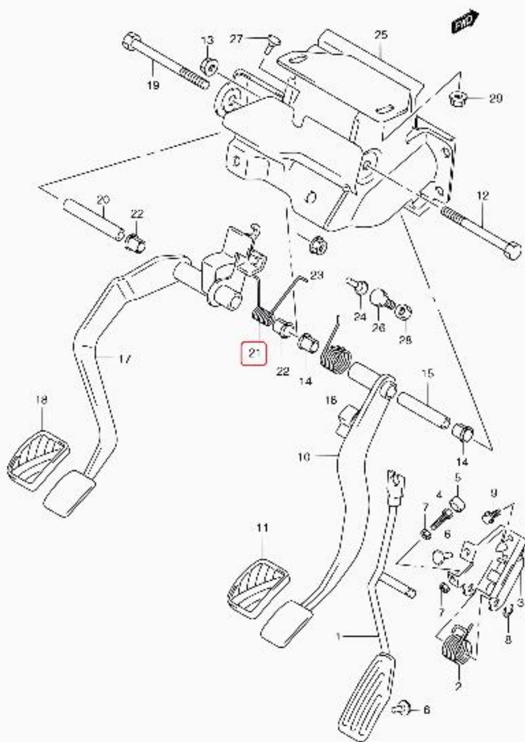
SN4 3V.7 E06_C60 PEDAL/PEDAL BRACKET
