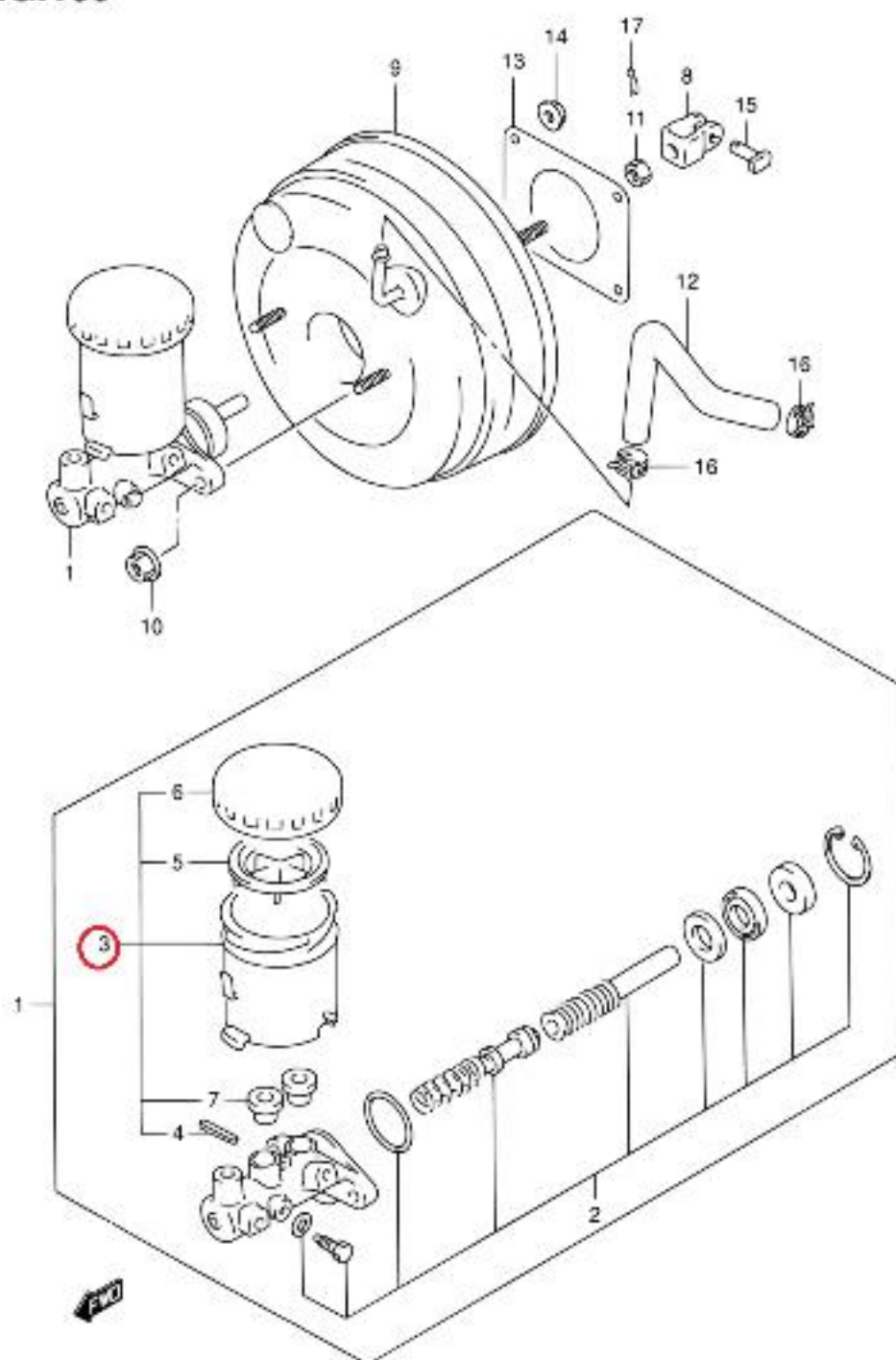
SV620-3 E01_169 BRAKE MASTER CYL (RHD)
