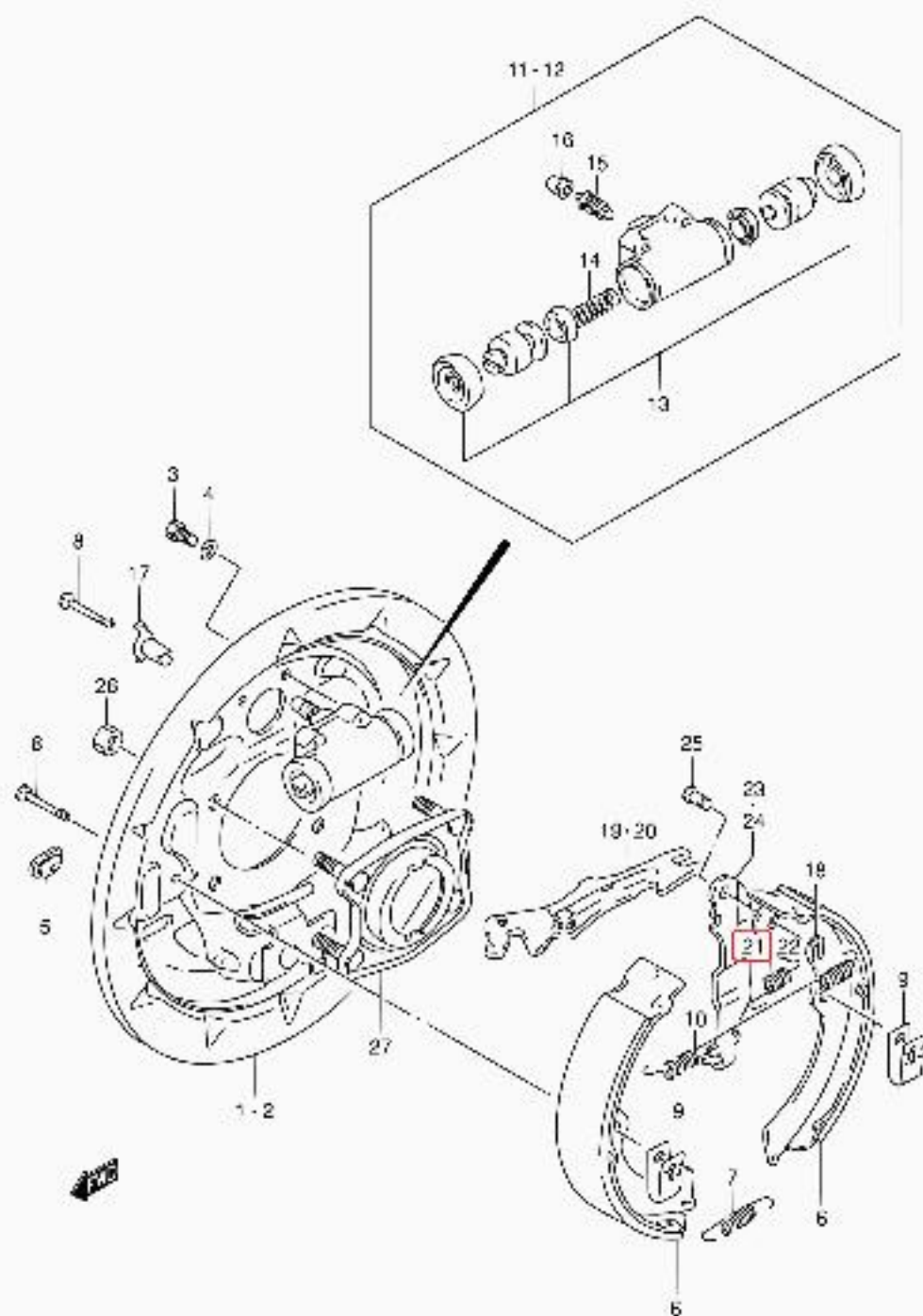
SE416 3DR E01 210 REAR BRAKE (1)
