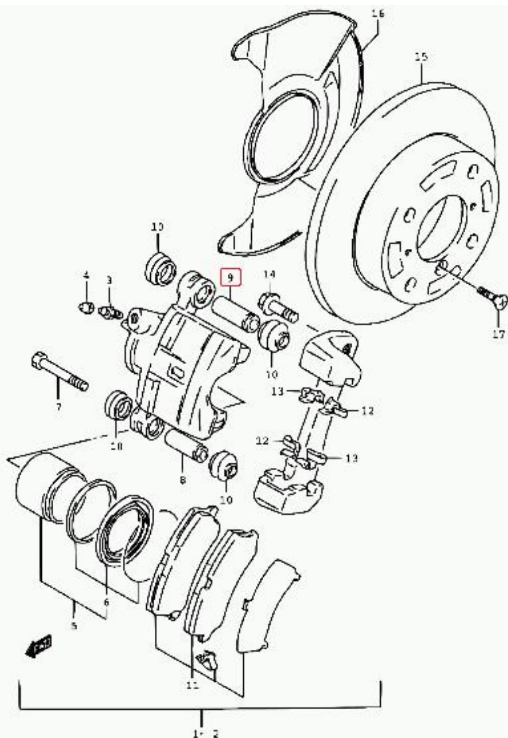
SY413-7 B01_219 FRONT WHEEL BRAKE (1)
