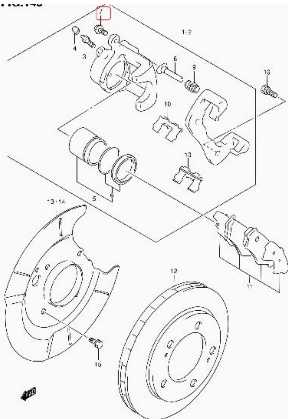
SQ416V-2 E22 140 FRONT WHEEL BRAKE
