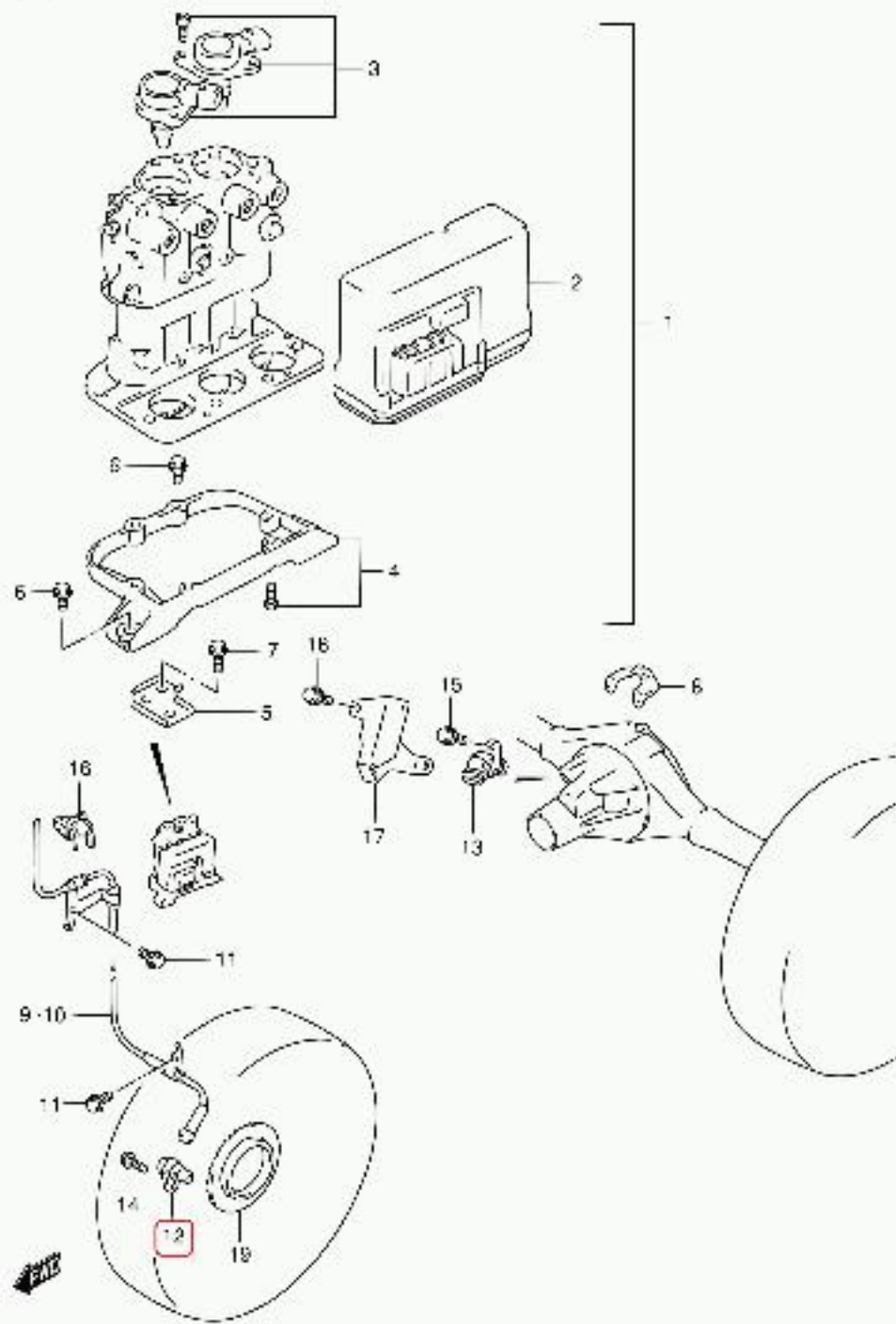
SE416 4 E01_161 ANTI LOCK BRAKE SYSTEM(ABS)
