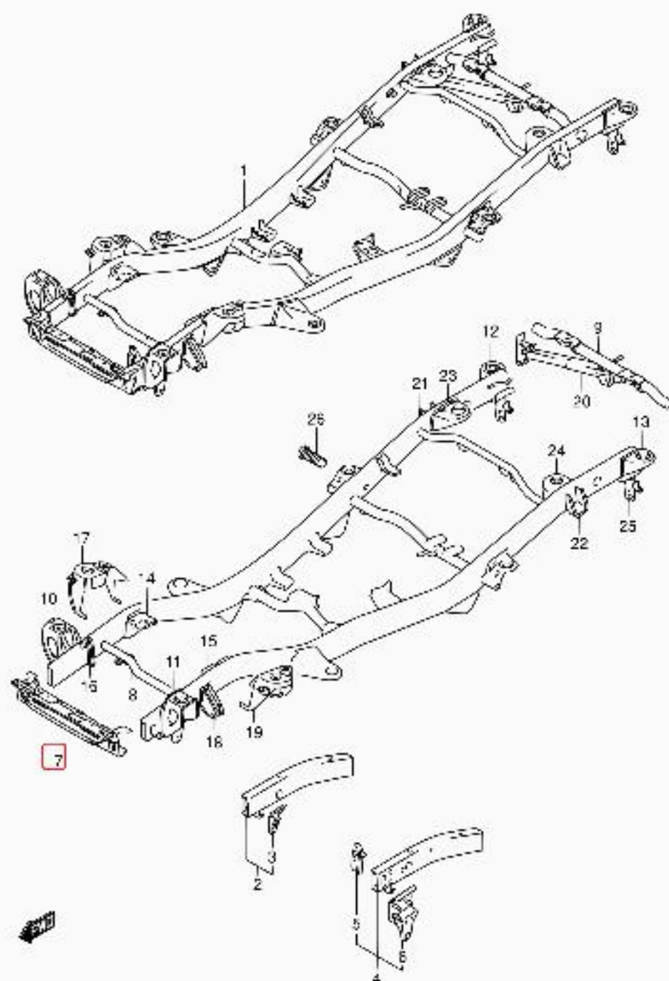
SA413V-5 E22 146 CHASSIS FRAME (3)
