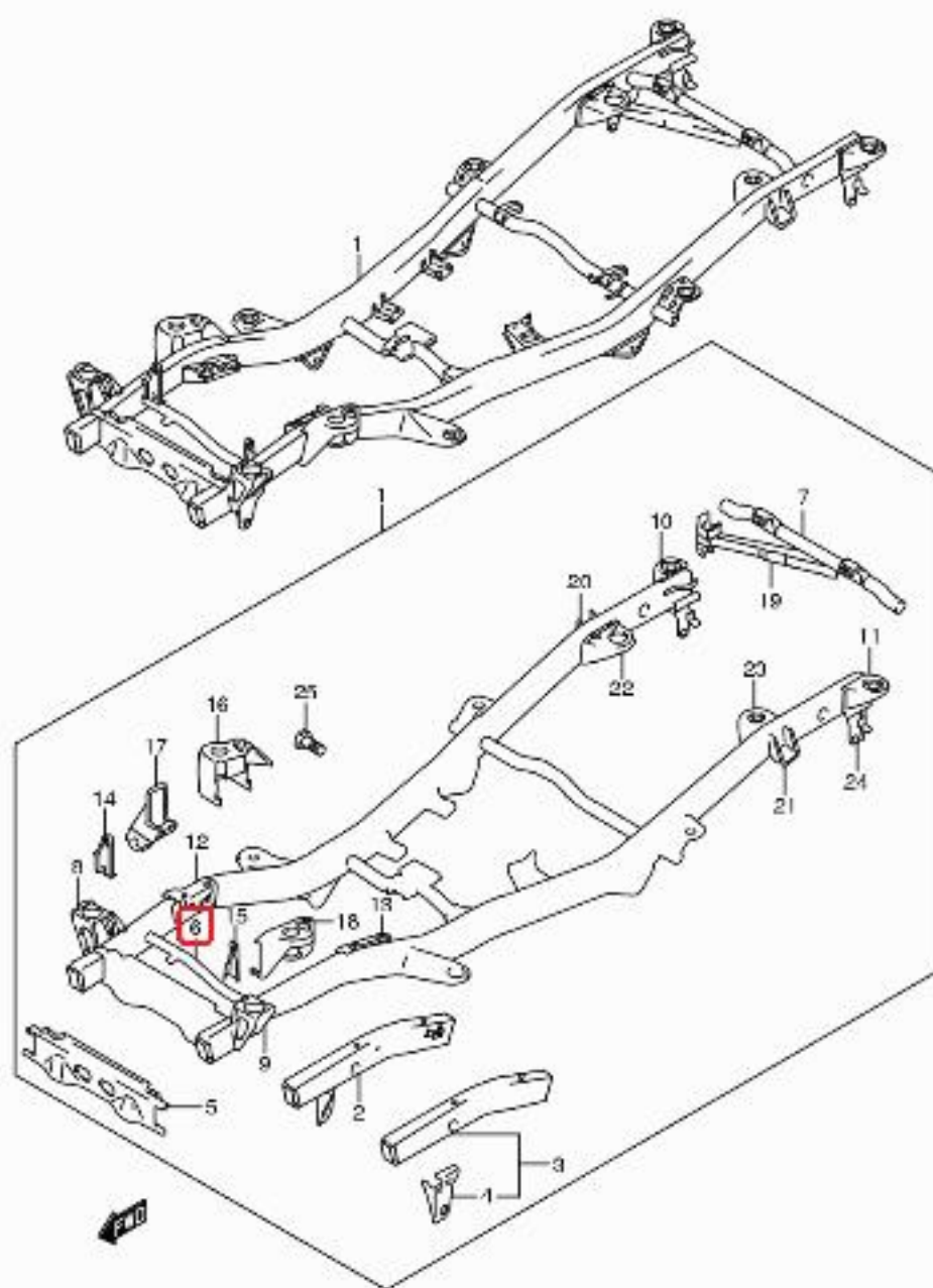
JB23W_570N CHASSIS FRAME
