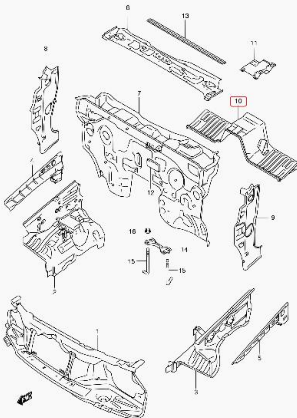
SN413V-7 EC6_071 FRONT BODY PANEL
