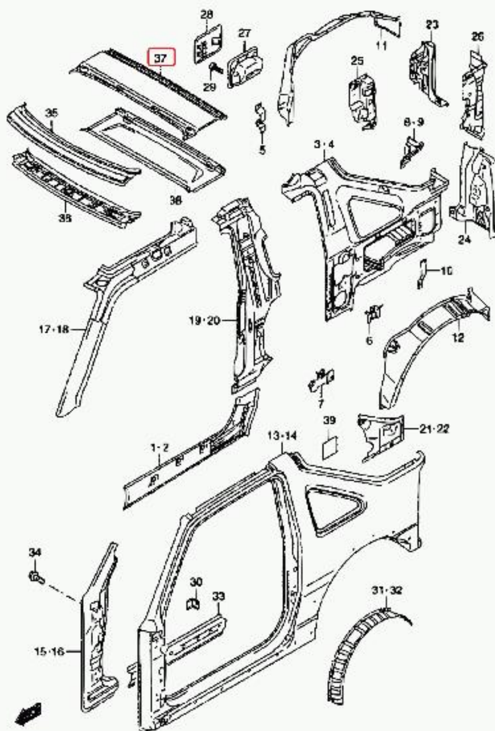
SN413-SN415D (TYPE 4)
