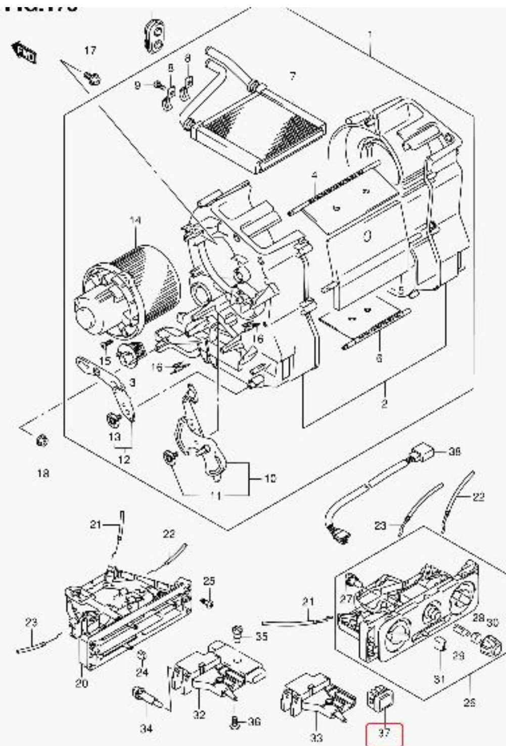
SM413V-2 E22 175 HEATER UNIT (SM413V:LHD)
