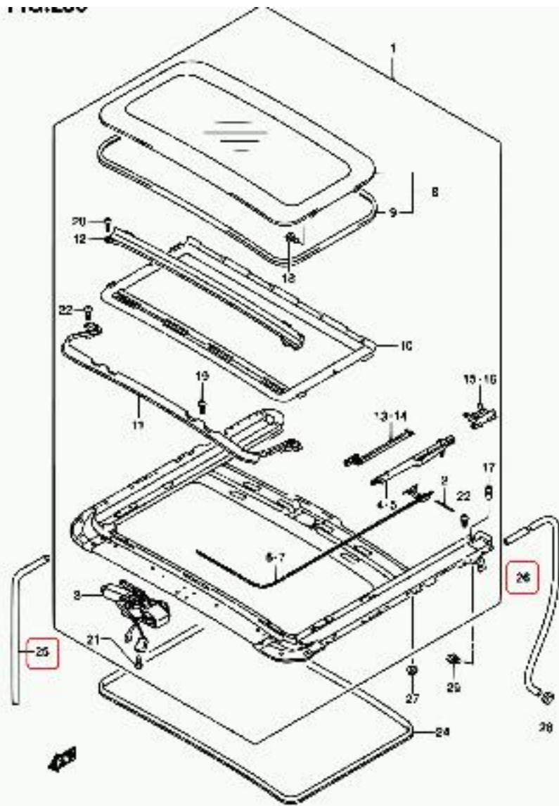
SQ420W-2 E22 256 SLIDING ROOF(W/SUN ROOF)
