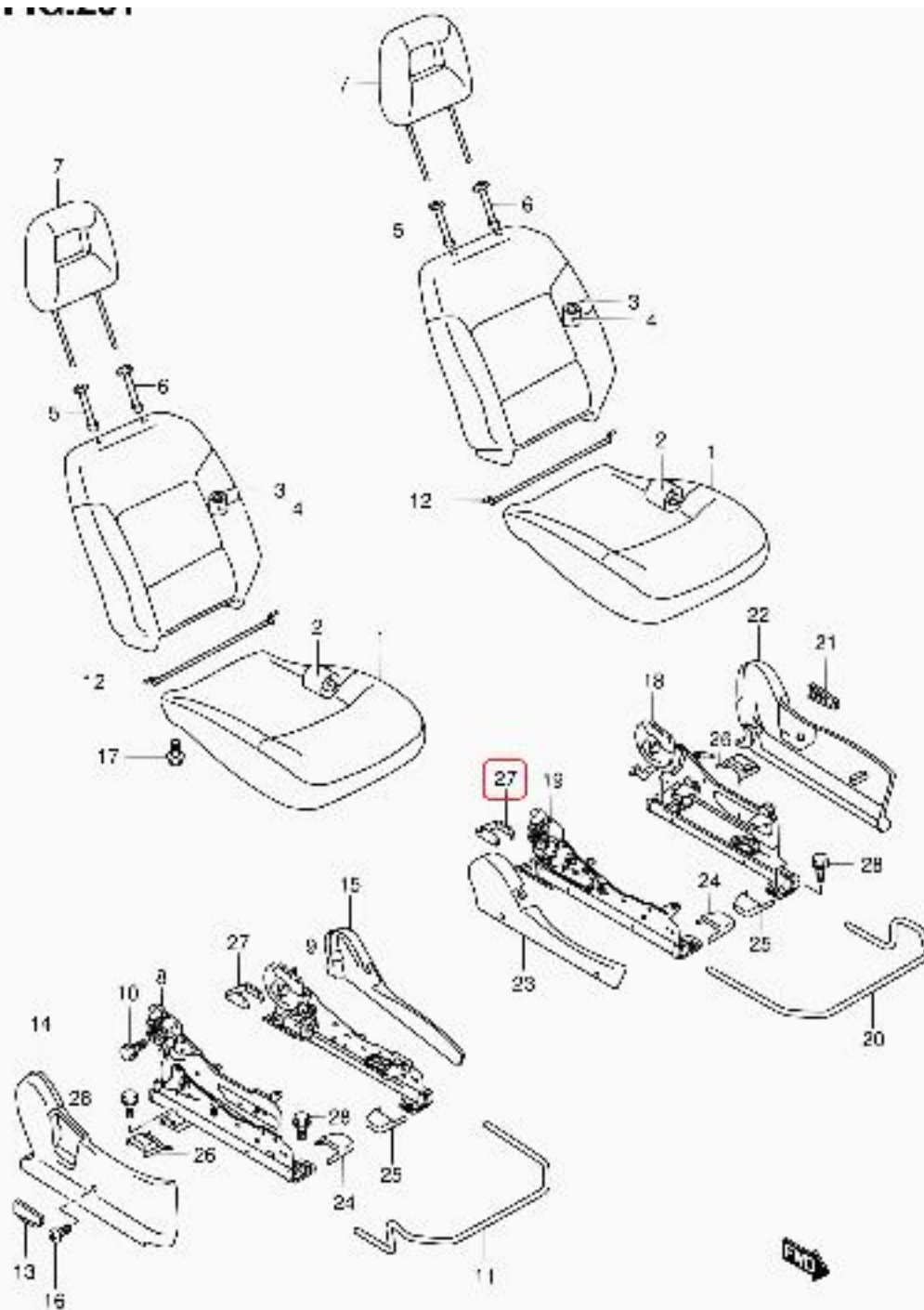
SM413V-2 E22 201 FRONT SEAT (JX)
