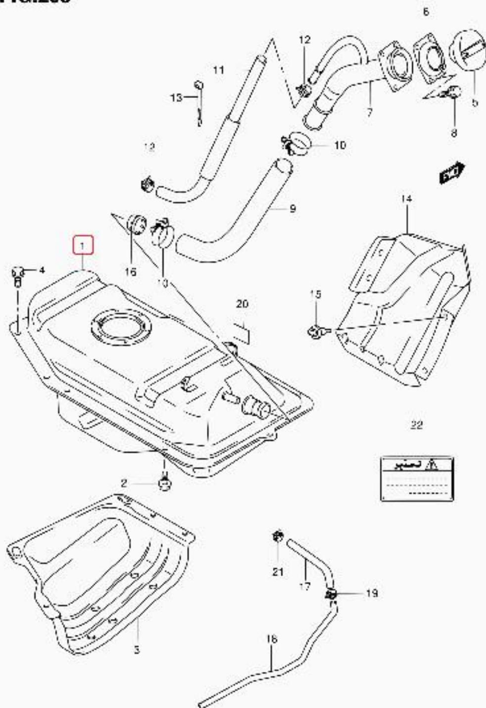
SA413V-2 E22 208 FUEL TANK (*)
