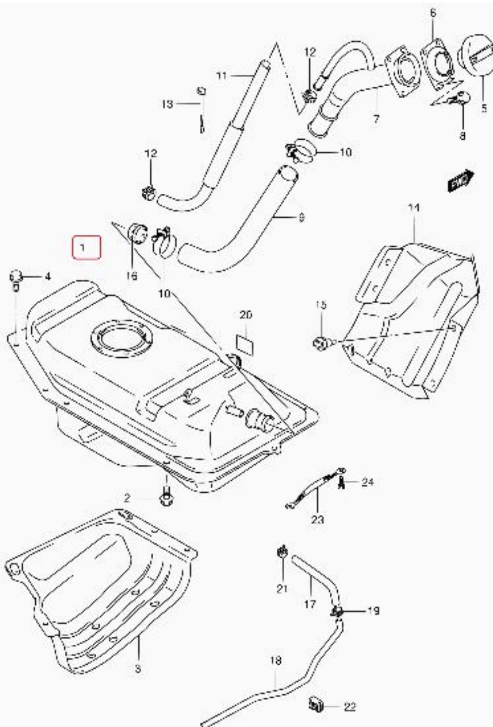
SN113V-7 E06_101 FUEL TANK
