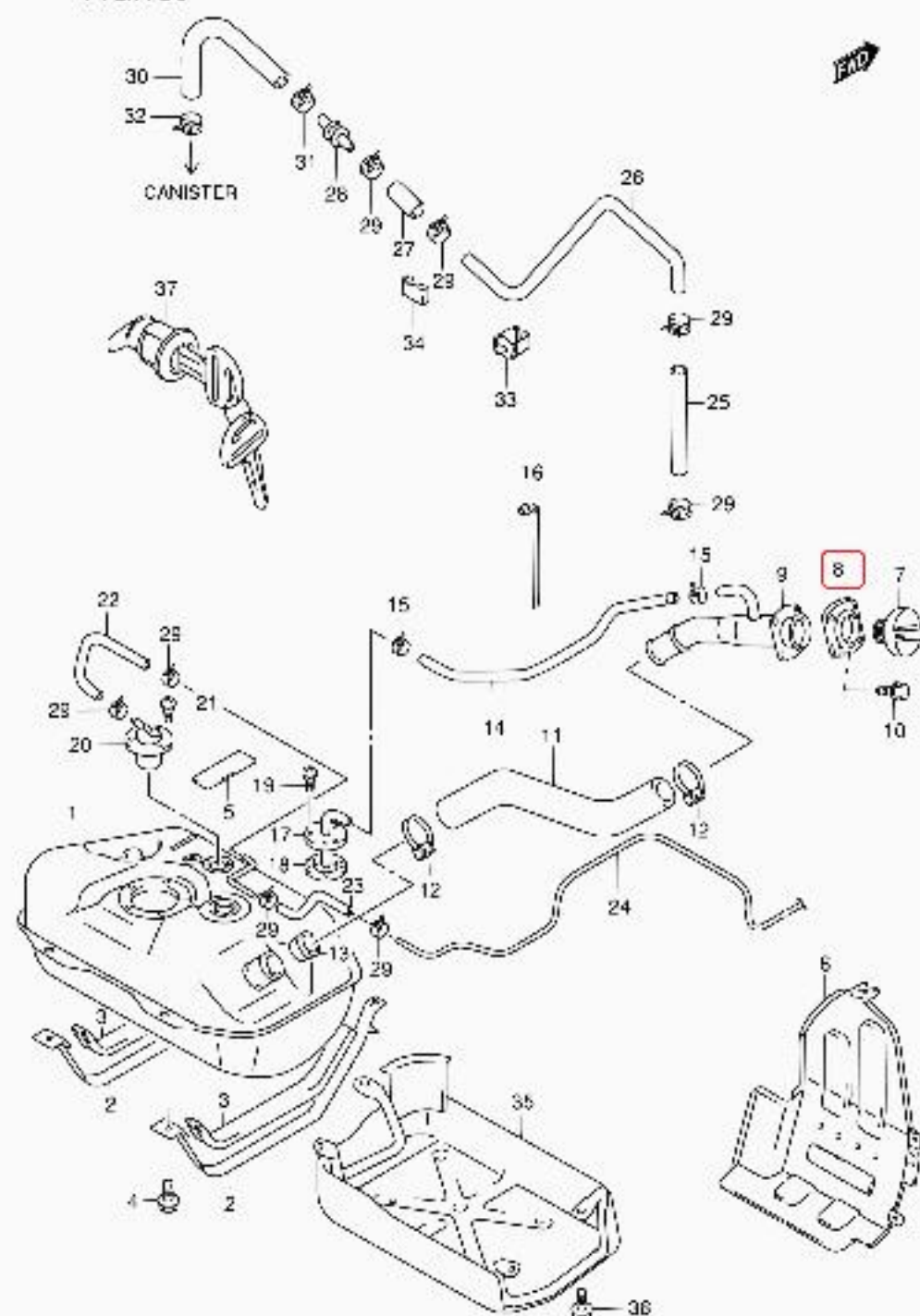
SQ420Q E22 160 FUEL TANK
