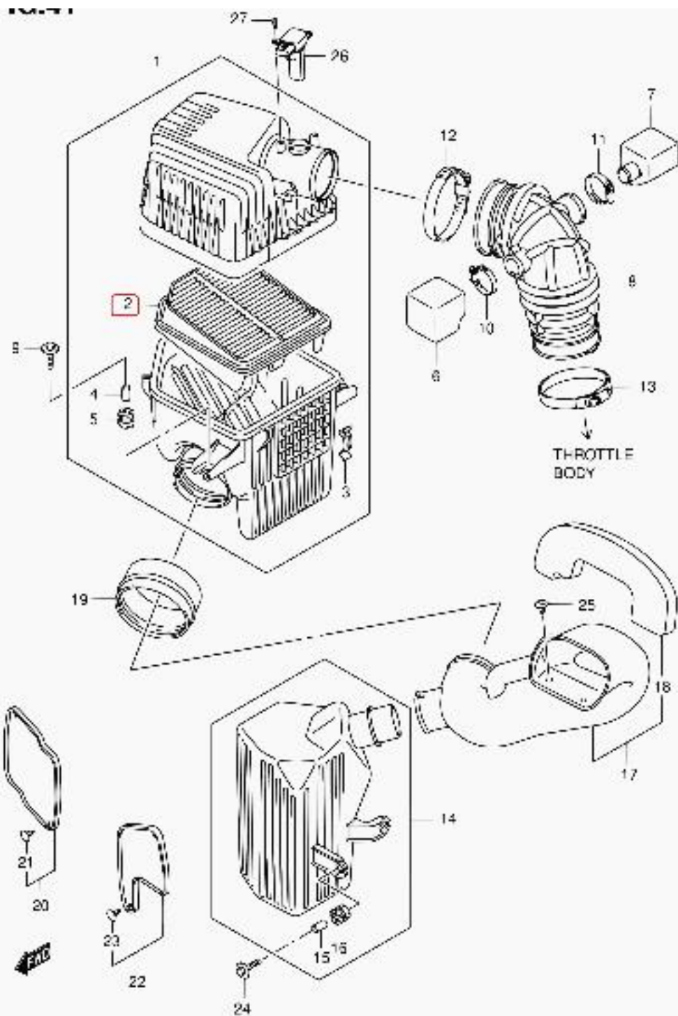
JB420W-4 E22 041 AIR CLEANER (2)
