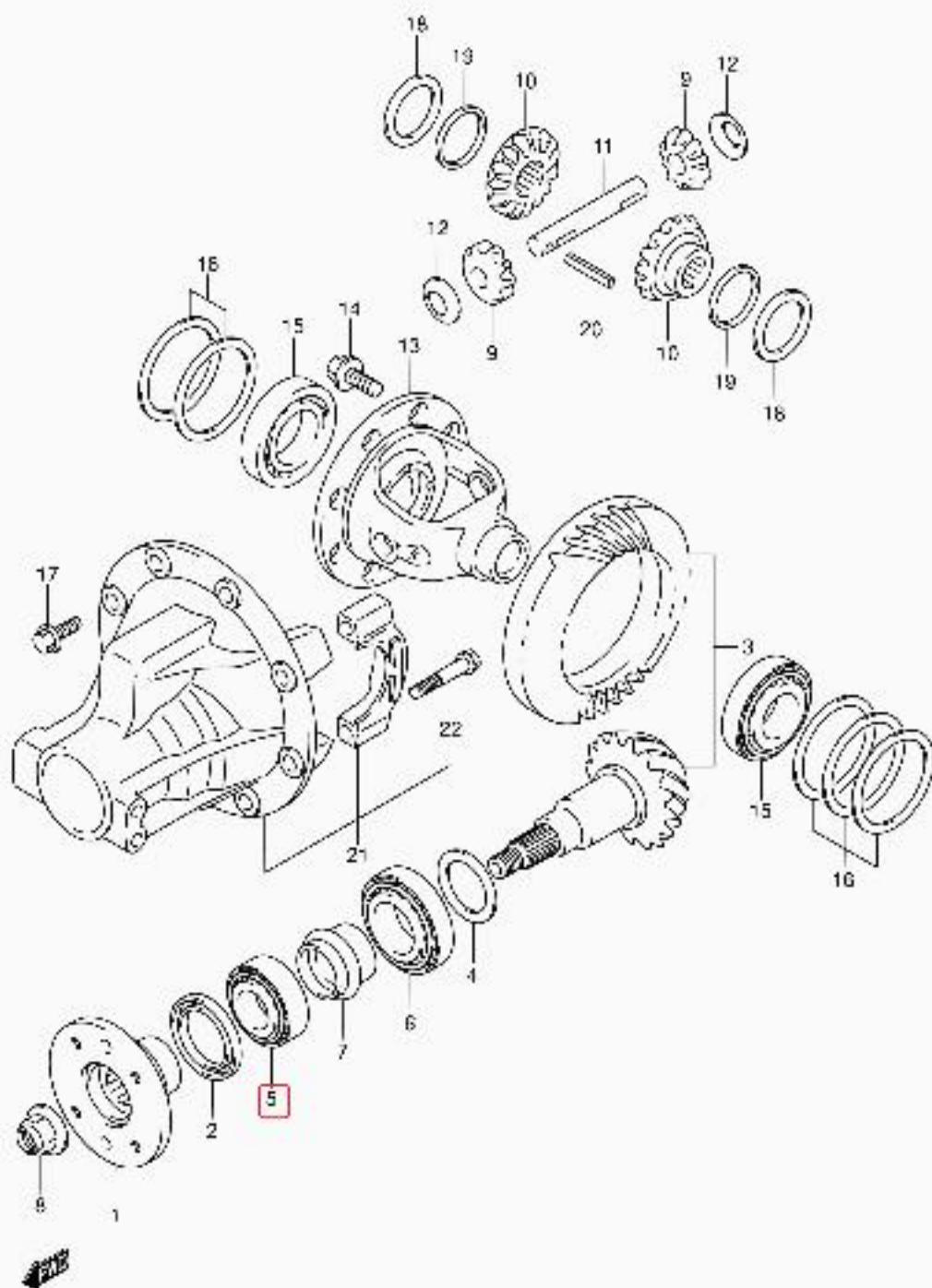
RM413 E22 087 REAR DIFF GEAR (4WD)
