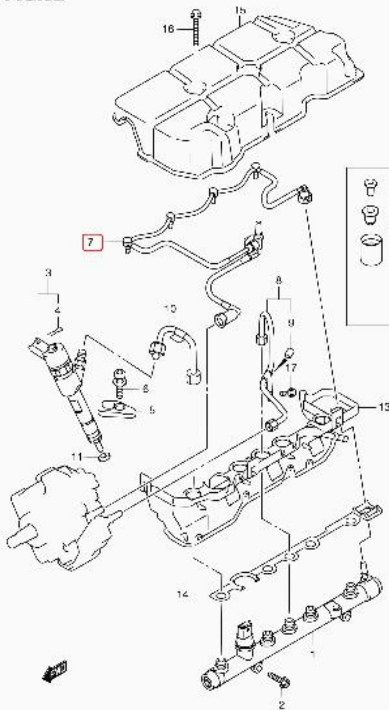
JB420W-1 E22_062 DELIVERY PIPE (3)
