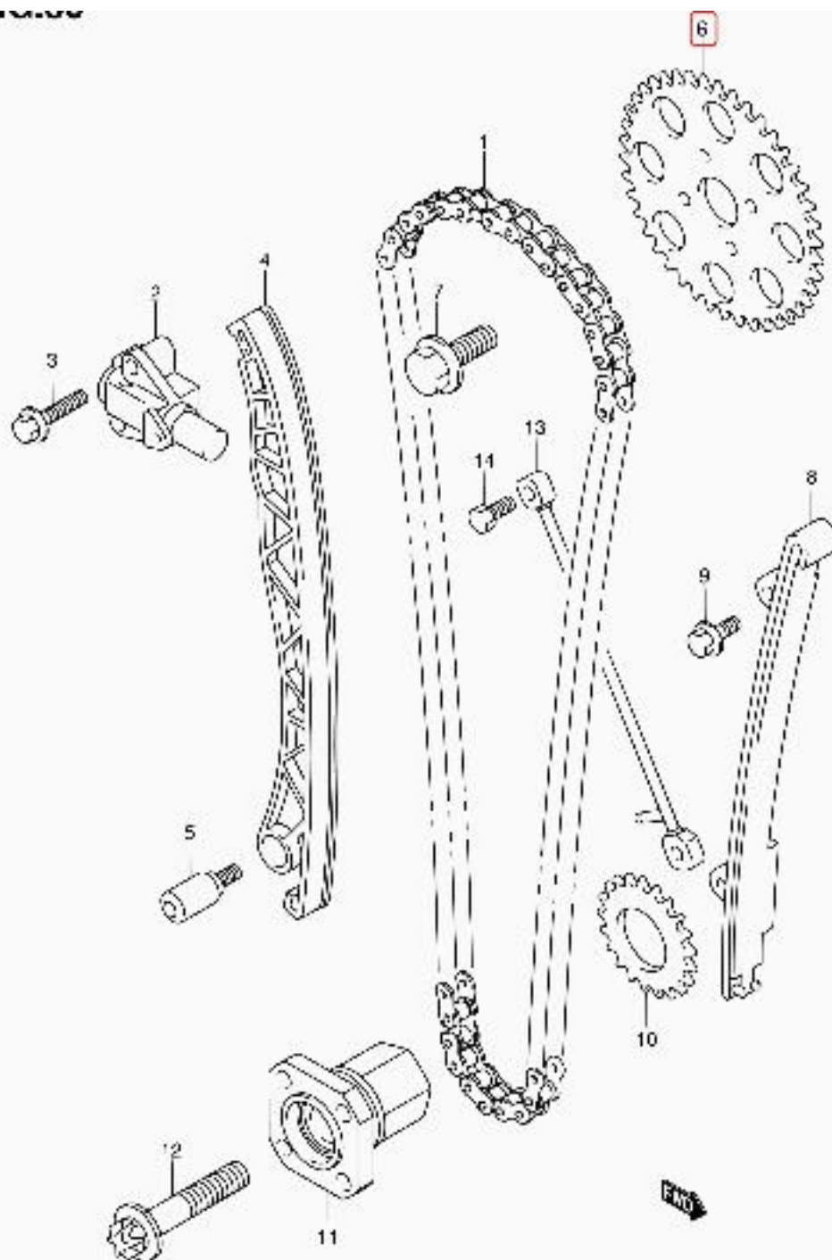
RS413 E22 030 CAM CHAIN (RS413D)
