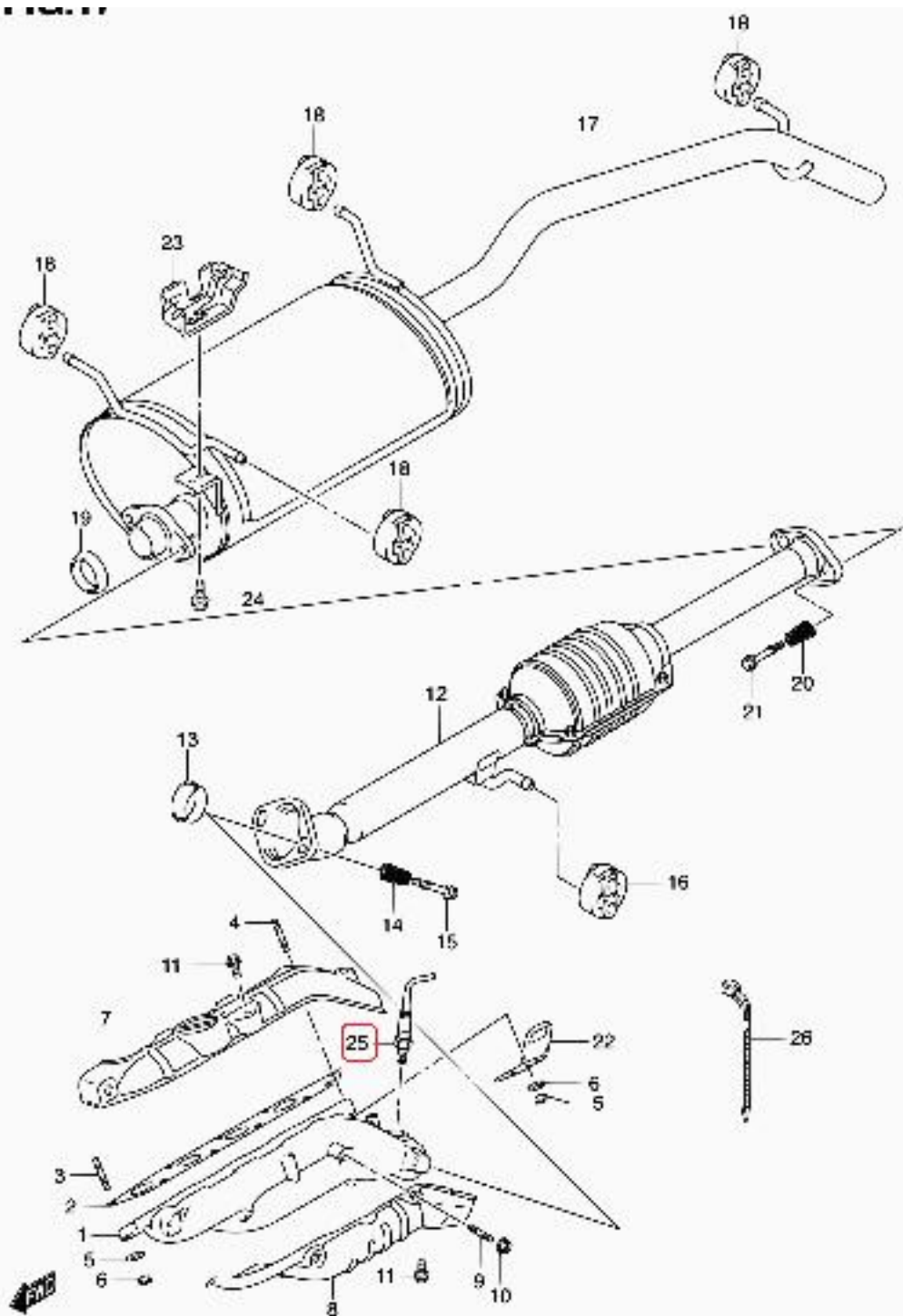
GC415T GC416T E01_017 MUFFLER (2)
