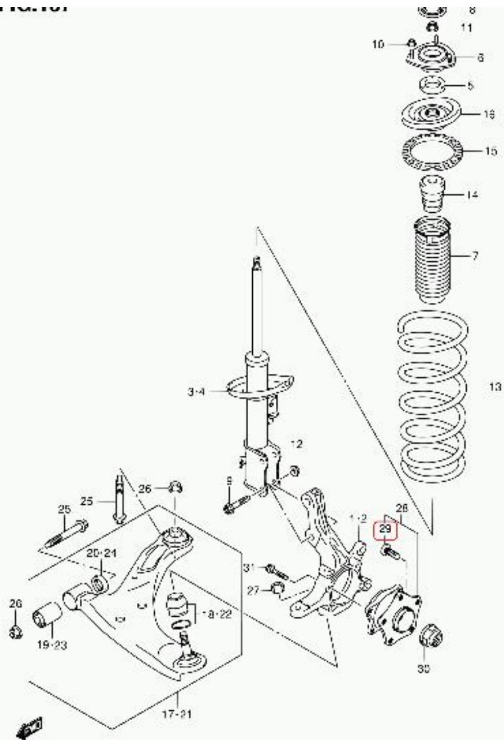
JB415X-4 E22 137 FRONT SUSPENSION
