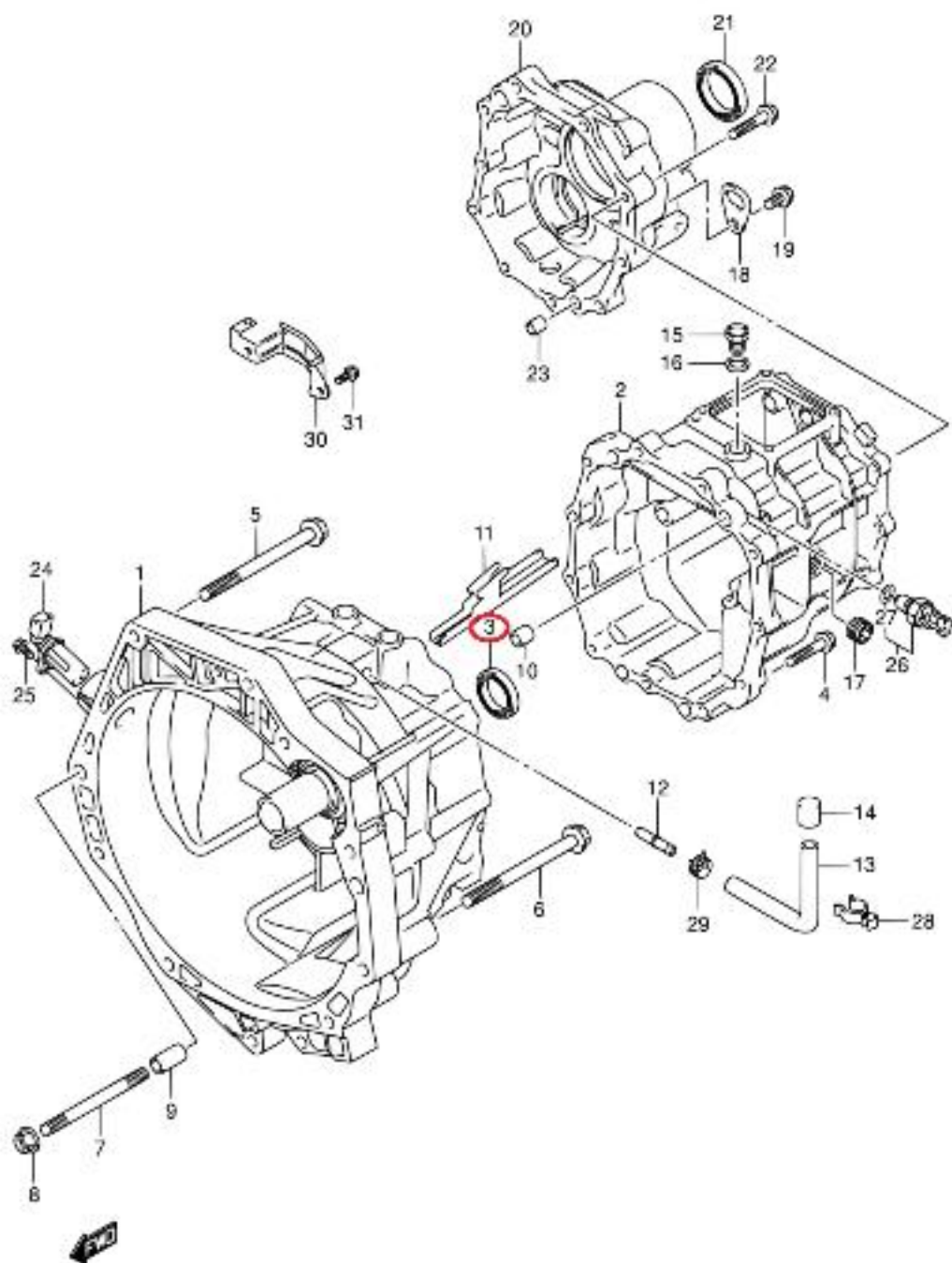
SN413V-5 E22 058A MT TRANSMISSION CASE (3)
