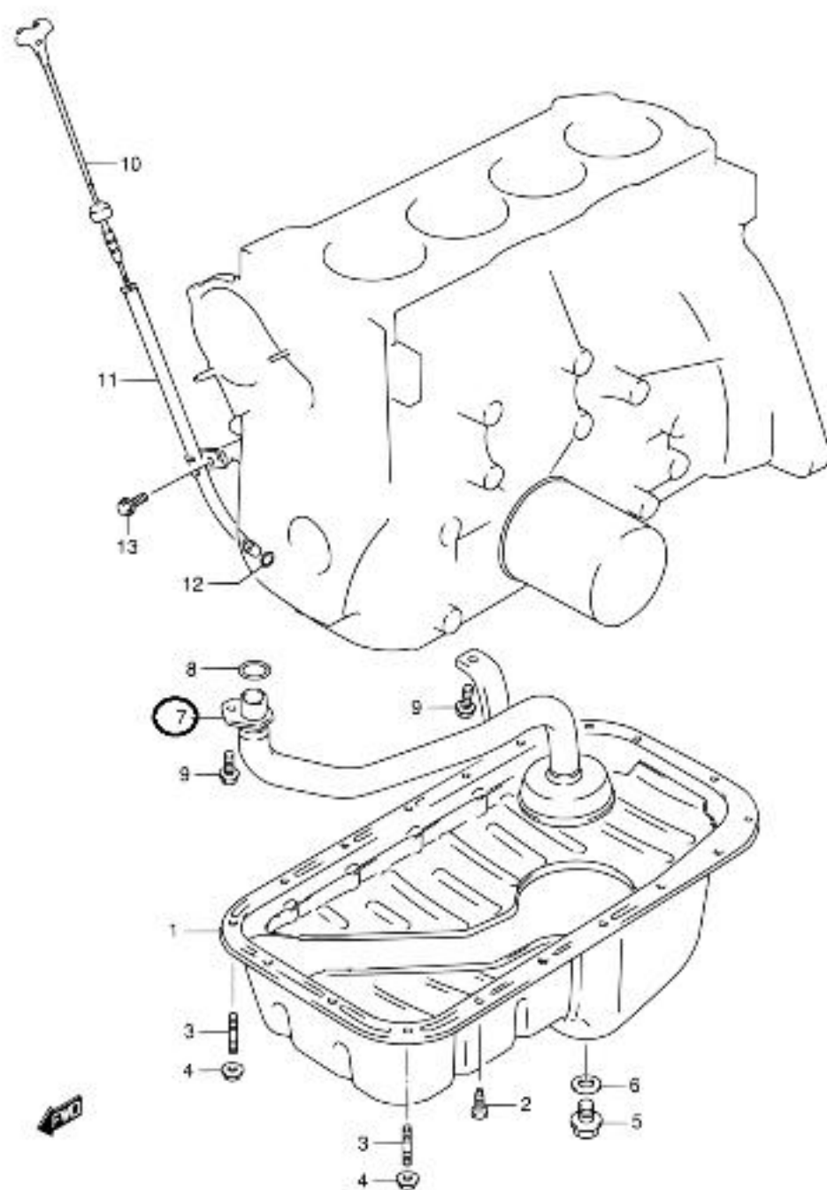
SE416 3DR E01 007 OIL PAN
