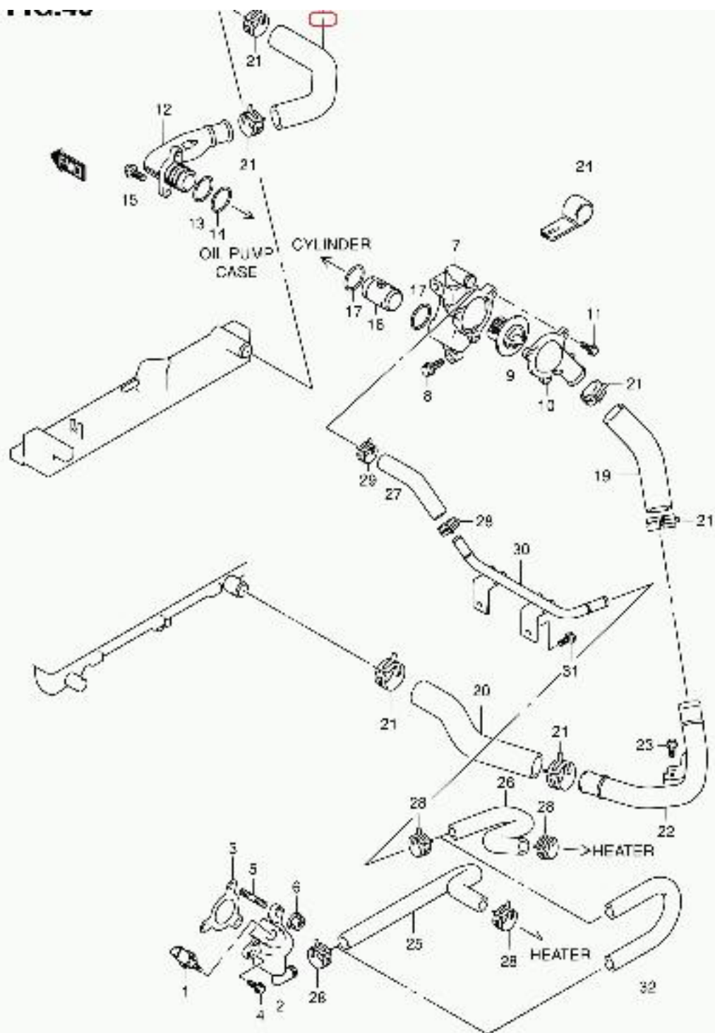
SN413V-2 E22 040 WATER HOSE (SN413V)
