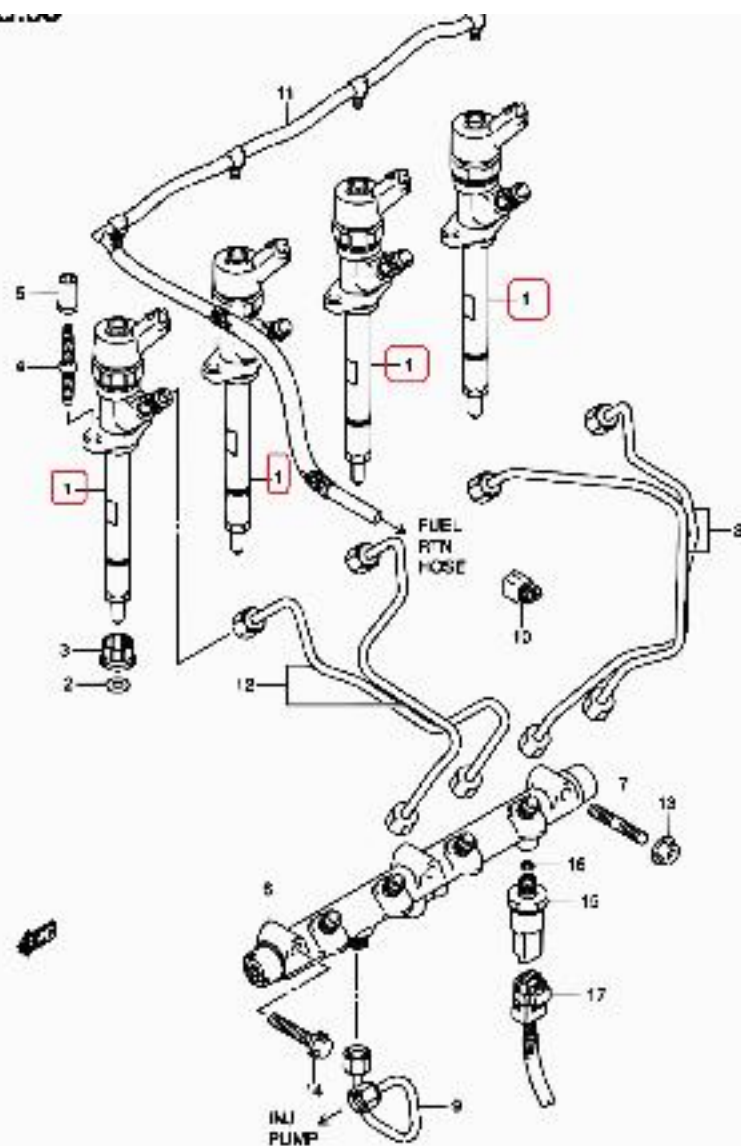
SQ420W-3 E22_058 DELIVERY PIPE (SQ420WD)
