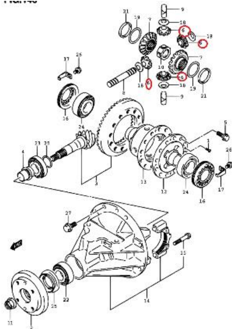
BQ420W-2 E22_146 REAR DIFF GEAR (BQ420WD:RHS:NT)
