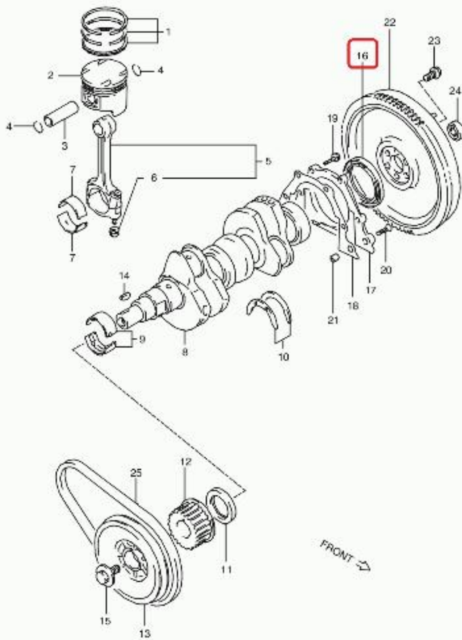
PG6SS_121 CRANKSHAFT
