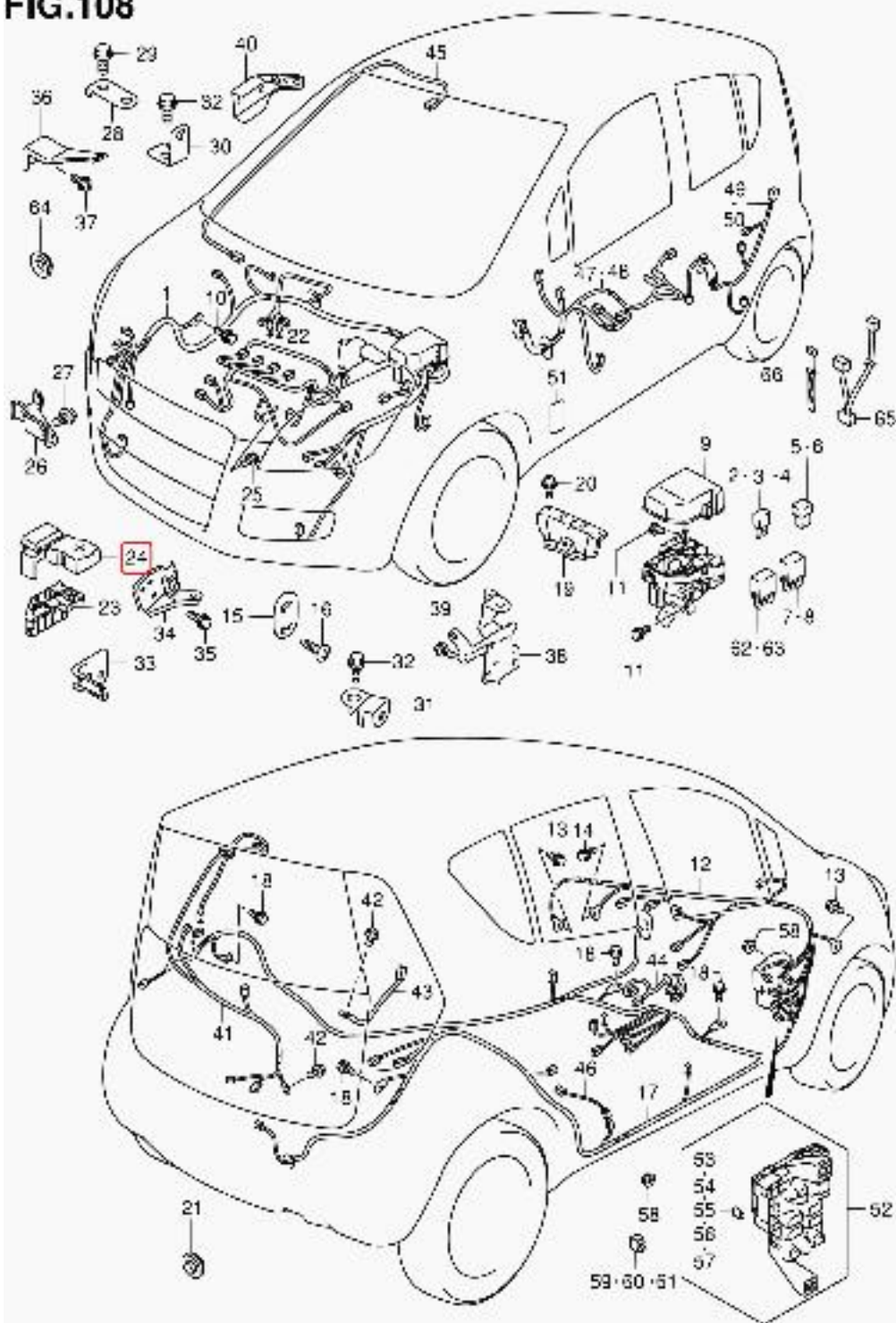
A5B310 E22 '08 WIRING HARNESS (1)
