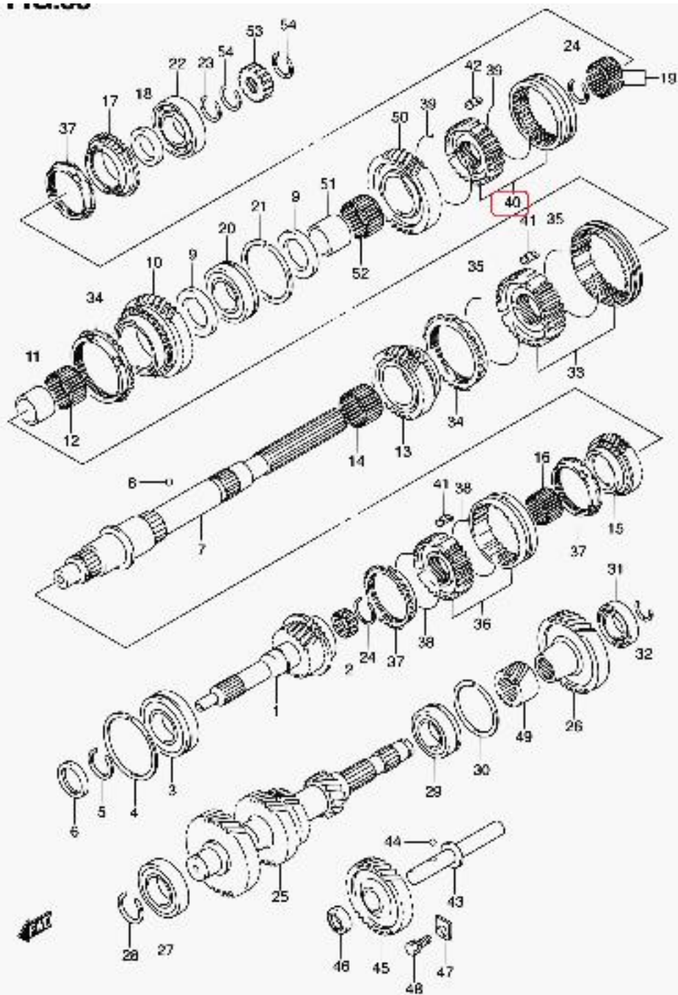
GC415T GC416T E01_003 MT TRANSMISSION GEAR (1)
