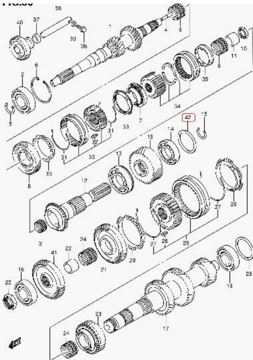
JB420W E22 050 MT TRANSMISSION (MT:JB420W)
