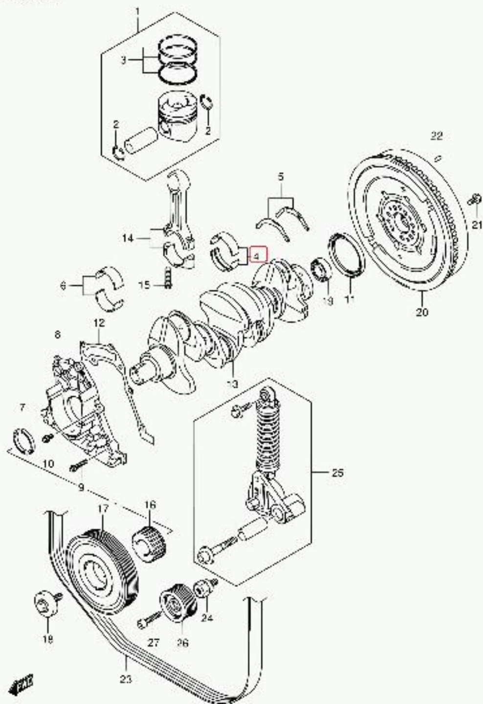
JB420W-4 E22 024 CRANKSHAFT (4)
