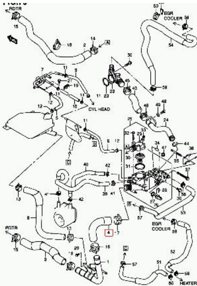
SQ420W-3 E22_070 WATER HOSE (SQ420W-3)
